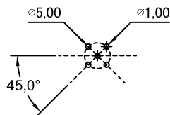
5 Pin Female Connector Female Pin PCB Layout
