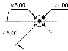
5 Pin Male Connector Male Pin PCB Layout
