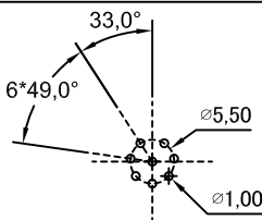
8 Pin Female Connector Female Pin PCB Layout
