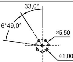
8 Pin Male Connector Male Pin PCB Layout
