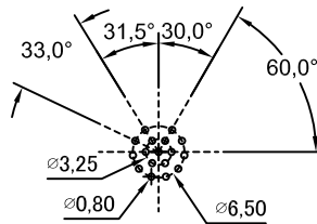
17 Pin Female Connector Female Pin PCB Layout
