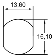
Recommended Panel Cut-Out
