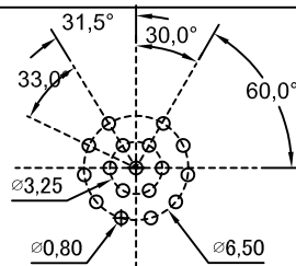
17 Pin Male Connector Male Pin PCB Layout
