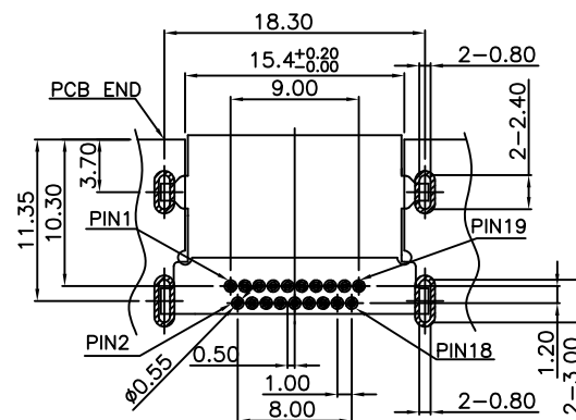
RECOMMEND PCB LAYOUT TOLERANCE: ±0.05 TOP VIEW
