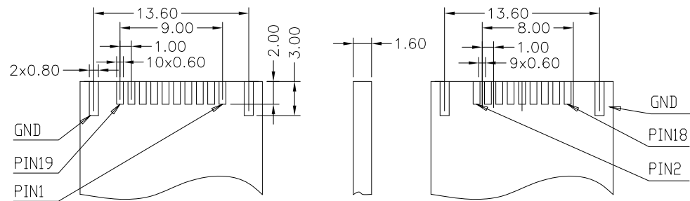
RECOMMENDED PCB LAYOUT2 T=1.60 GENERAL TOLERANCES:±0.05
