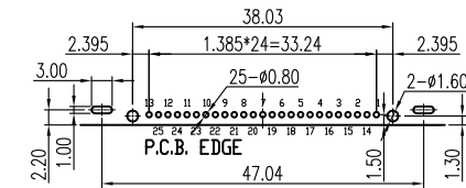
RECOMMENDED P.C.B LAYOUT INSPECTION DIMENSION:(A)~(I)
