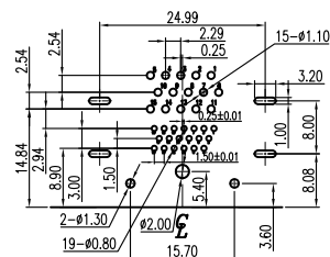
RECOMMENDED P.C.B LAYOUT INSPECTION DIMENSION:(A)~(M)
