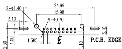
RECOMMENDED P.C.B. LAYOUT INSPECTION DIMENSION(A)~(I)
