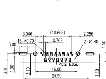
RECOMMENDED P.C.B LAYOUT INSPECTION DIMENSION:(A)~(K)
