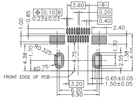
RECOMMENDED PCB LAYOUT(XX±0.05) CONNECTOR SIDE(TOP VIEW)
