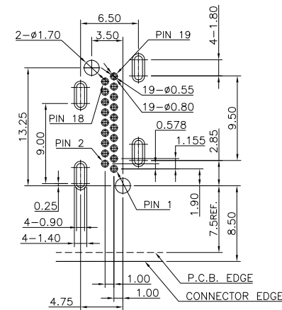
RECOMMENDED PCB LAYOUT (TOP VIEW) TOLERANCE: ±0.05mm
