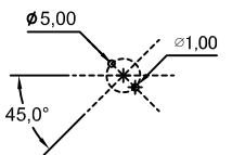
2 Pin Female Connector Female Pin PCB Layout
