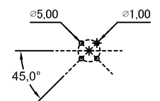
4 Pin Female Connector Female Pin PCB Layout
