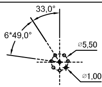
8 Pin Female Connector Female Pin PCB Layout
