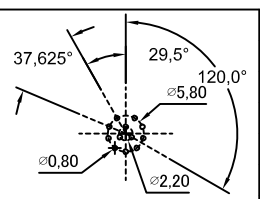
12 Pin Male Connector Male Pin PCB Layout
