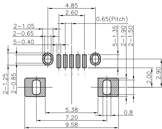
RECOMMENDED PCB LAYOUT(TOP VIEW) GENERAL TOLERANCES:±0.05
