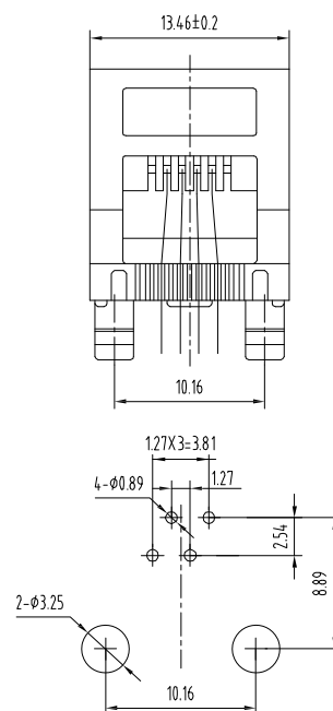
PC Board Layout Component Side Shown
