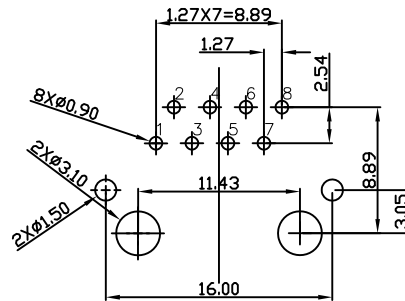
PC BOARD LAYOUT T=1.6mm COMPONENT SIDE SHOW
