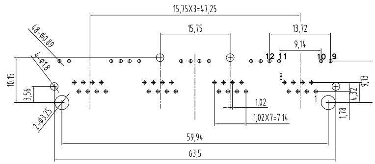
PC Board Layout Component Side Showr
