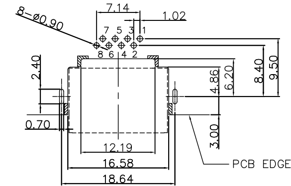
W/LED RECOMMENDED PCB LAYOUT COMPONENT SIDE(t=1.6mm, tol:±0.05)
