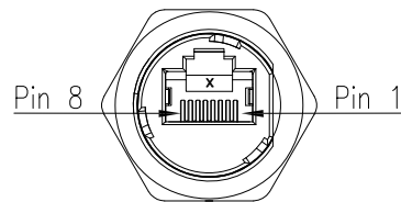
Pin Assignments Front View
