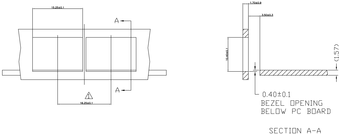
RECOMMENDED BEZEL DESIGN
