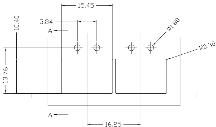
RECOMMENDED BEZEL DESIGN
