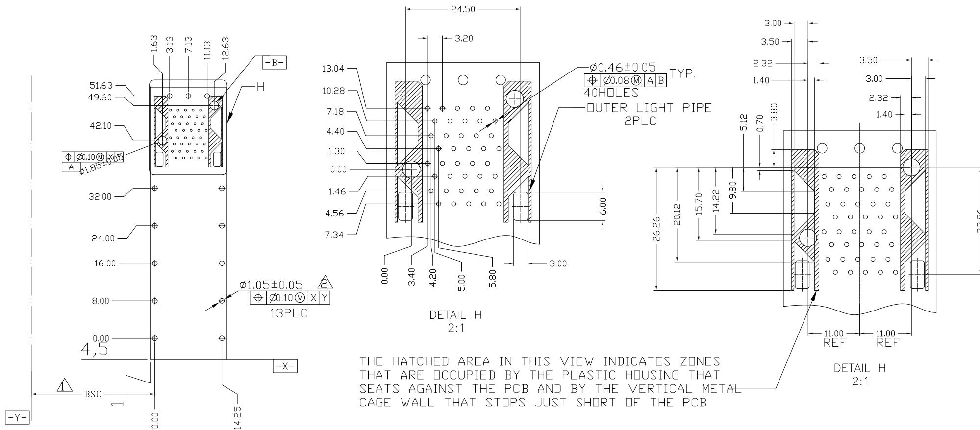
RECOMMENDED PCB CONFIGURATION
