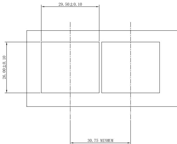
BEZEL CUT-OUT CENTER SPACING DETAIL BZZEL THICKNESS:0.8~2.6
