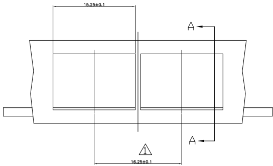
RECOMMENDED BEZEL DESIGN
