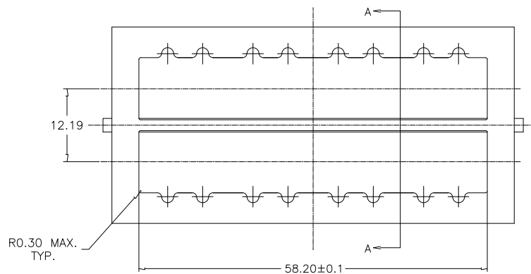
RECOMMENDED BEZEL DESIGN BELLY TO BELLY APPLICATIONS
