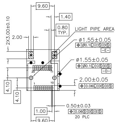
DETAIL H RECOMMENDED CONNECTOR LAYOUT 4X INDIVIDUALLY
