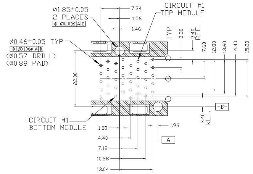
TERMINAL TAIL PATTERN SCALE 2:1
