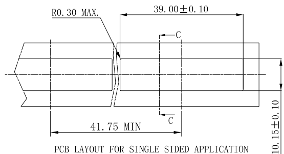
PCB LAYOUT FOR SINGLE SIDED APPLICATION
