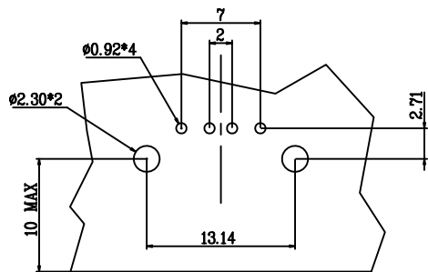
PC BOARD FOOTPRINT
