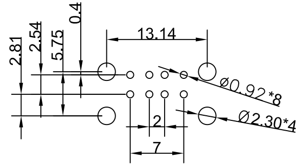
PC BOARD FOOTPRINT
