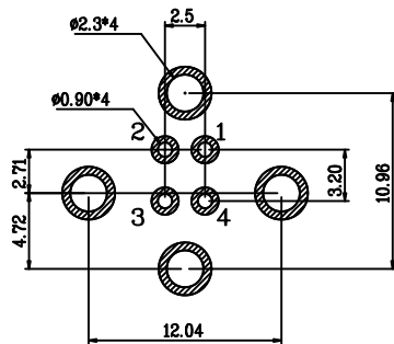
PC BOARD FOOTPRINT
