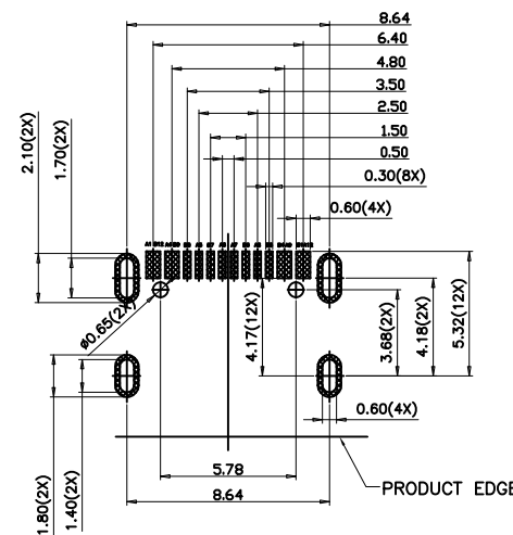
RECOMMENDED PCB LAYOUT(TOP VIEW) THICKNESS 0.80MM;DEFAULT TOLERANCE:±0.05
