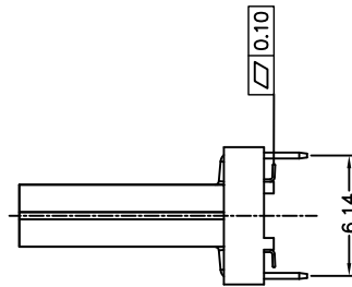
WITHOUT COVER
